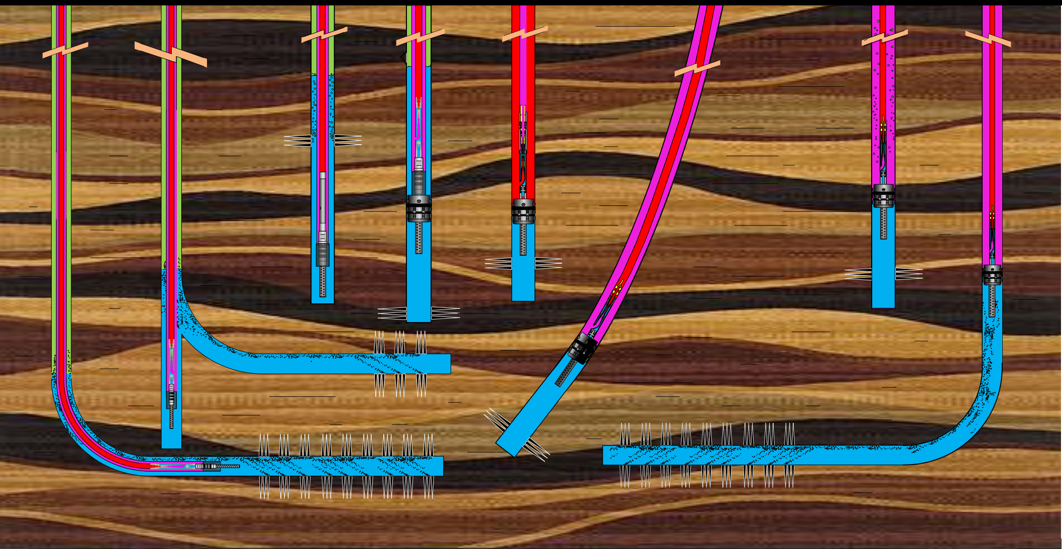
Horizontal Gas Well Dewatering Producing Inside Horizontal
